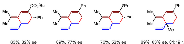
Scheme 21 \text{Pd}(0) -catalyzed asymmetric intermolecular [4+2] cycloadditions of vinylallenes and 1,3-dienes.
