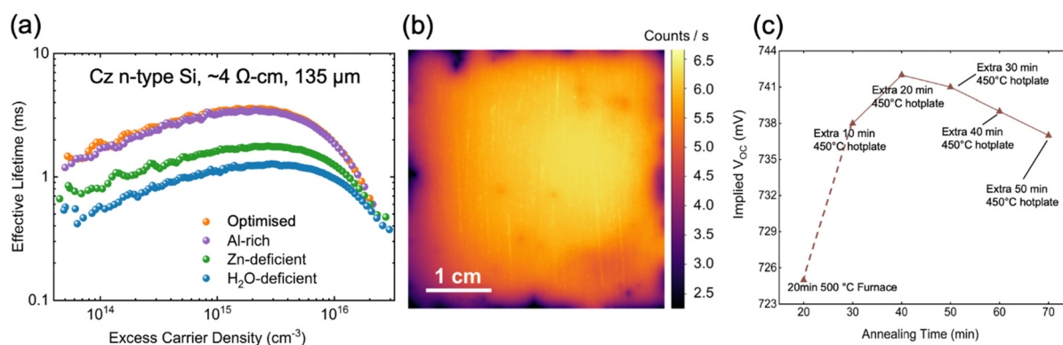
Fig. 2 (a) Effective lifetime vs. excess carrier density of samples from the four different pressure profiles; (b) PL image of the champion sample from the optimised recipe; (c) iV_{OC} values vs. annealing time for the champion sample undergoing post-deposition annealing at 450 °C.
