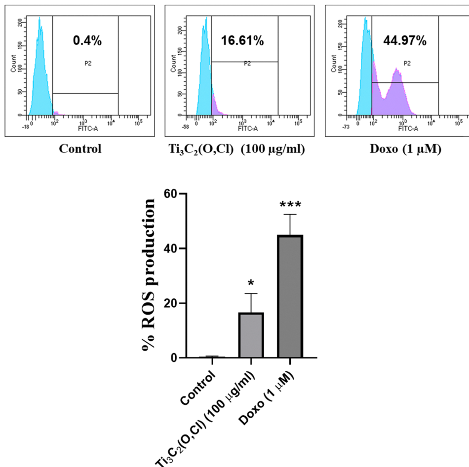
Fig. 8 MXene and Doxo induced reactive oxygen species (ROS) production in HEK-293 cells for 24 h. Data are shown as mean \pm SD ( n = 3 ) of three independent experiments. *** p < 0.001 and * p < 0.05 vs. control.
