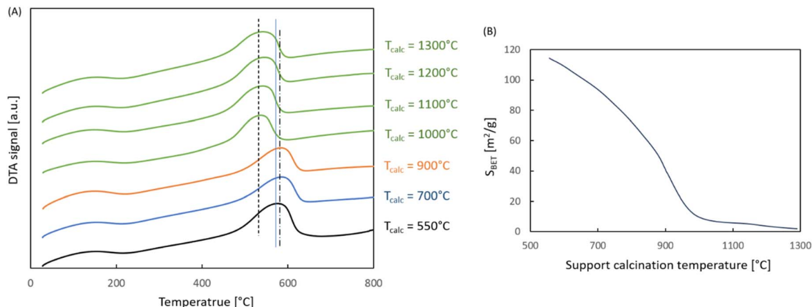
Fig. 1 Catalyst properties: (A) soot combustion activity results of Ag/alumina samples; initial alumina calcination temperature is indicated on the right; solid line: T_{\text{max}} with Ag/Al-550, dashed-and-dot line: highest T_{\text{max}} with Ag/Al-900, and dashed line: lowest T_{\text{max}} with Ag/Al-1000, and (B) surface area results.
