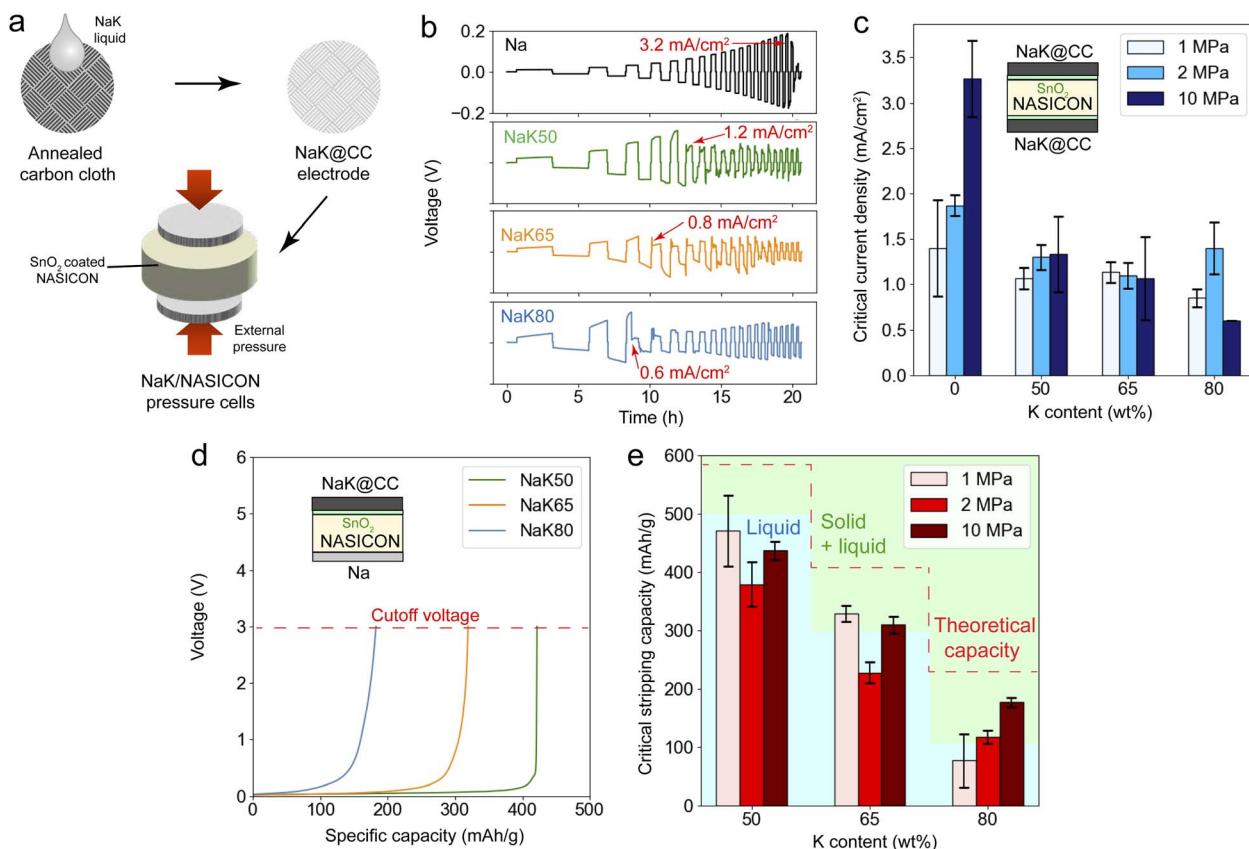
Fig. 1 (a) Assembling solid-state NaK/NASICON pressure cells for electrochemical testing with free-standing NaK@CC electrodes and \text{SnO}_2 -coated NASICON pellets. (b) Critical current density (CCD) tests on Na, NaK50, NaK65 and NaK80 symmetric cells collected at 10 MPa external pressure. (c) CCD results collected on the same group at different external pressures. (d) Critical stripping capacity tests on NaK50, NaK65 and NaK80 collected with asymmetric cell setup at 10 MPa external pressure. (e) Critical stripping capacity of NaK alloys collected at different external pressures. Background color indicates capacity regions where different bulk phase compositions in NaK anodes are expected, based on Na–K phase diagram.
