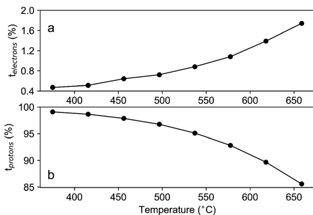
Fig. 10 (a) Extracted transport number of electrons in LNw16 under dry 5% H 2 atmosphere from DC polarization measurements; (b) estimated transport number of protons in LNw16 under dry 5% H 2 /N 2 atmosphere.
