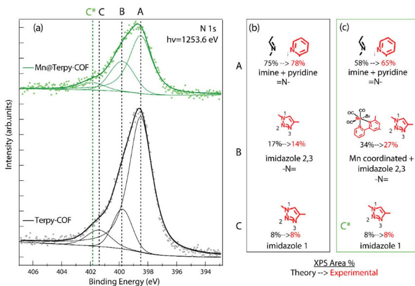
Fig. 5 (a) XPS spectra of the N 1s peak region of Terpy-COF (black) and Mn@Terpy-COF (green). Dots correspond to experimental points and continuous lines to the deconvolution in different components and the background. Vertical dotted lines indicate the binding energy positions of the components. Panels (b) and (c) show the origin of each N 1s component. Data obtained with a Mg K\alpha (1253.6 eV) photon source.
