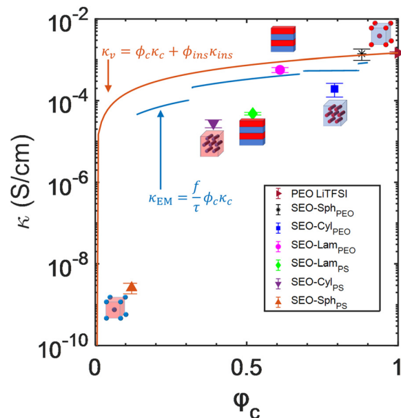
Fig. 9 Measured and predicted ionic conductivities of SEOs with salt at 90 °C ( r = 0.085 \text{ mol}_{\text{LiTFSI}} \text{ mol}_{\text{PEO}}^{-1} ). The blue line represents the effective medium prediction, \kappa_{\text{EM}} (eqn (1)), in which SEO-Sph PS is approximated as a perfect insulator. The orange line represents a simple volume-weighted average model of the conductivity, \kappa_v (eqn (7)), of PEO/LiTFSI and polystyrene at 90 °C. The equations for each of these models are shown in blue and orange on the figure, respectively.
