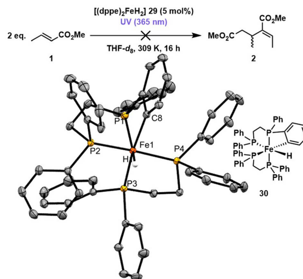
Scheme 3 Using [(dippe)_2FeH_2] 29 as catalyst for methyl crotonate 1 dimerisation under UV (365 nm) irradiation for 16 hours yielded no ( E ),( Z )-2-ethylidene-3-methylpentanedioate 2 . Crystals suitable for X-ray crystallography were grown from the reaction mixture at -35^\circ C and identified as [(dippe)FeH(Ph_2PCH_2CH_2PPh(C_6H_4))] 30 . Iron, carbon and phosphorus atoms on the molecular structures are coloured orange, grey and yellow respectively. Hydrogens have been omitted for clarity and thermal ellipsoids have been set at 50% probability.
