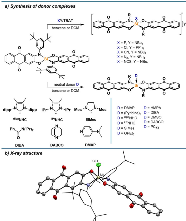
Fig. 5 (a) Synthesis of pentacoordinate silicon complexes with neutral and anionic donors. (b) Molecular structure of [1-Cl][PPh 4 ] determined by SCXRD analysis. Hydrogen atoms and the \text{PPh}_4 cation are omitted for clarity. Thermal displacement ellipsoids are displayed at the 50% probability level. Selected bond lengths [pm]: Si1–Cl1: 211.64(10), Si1–O1: 174.78(18), Si1–N1: 178.1(2). Selected bond angles [°]: N1–Si1–N1: 128.16(10), O1–Si1–O4: 177.74(9), N1–Si1–Cl1: 116.45(8), O1–Si1–Cl1: 91.53(7).
