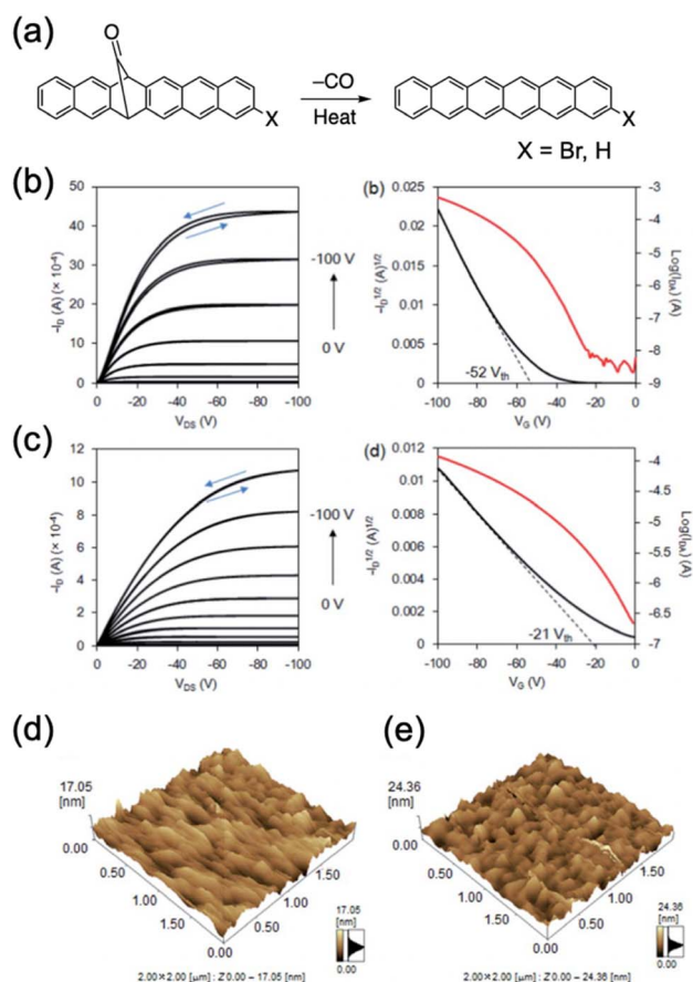
Fig. 30 (a) Synthetic route for brominated hexacene and pristine hexacene. (b) Vacuum-deposited thin-film OFETs based on brominated hexacene. Output (left) and transfer characteristics (right, V_{DS} = -100 V). (c) Vacuum-deposited thin-film OFETs based on hexacene. Output (left) and transfer characteristics (right, V_{DS} = -100 V). AFM images of thin films of (d) brominated hexacene and (e) pristine hexacene. Adapted with permission from ref. 110. Copyright 2018 Royal Chemical Society.
