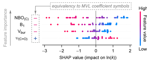
Same influence on predictions (MVL-NN)
