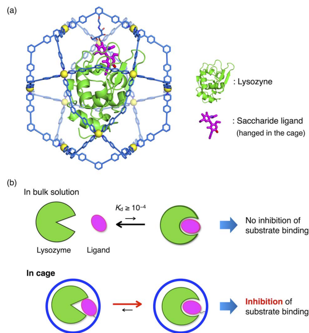
Fig. 1 Enhanced ligand binding to protein's active sites by confinement in coordination cages. (a) Lysozyme–saccharide complex encapsulated in a spherical M_{12}L_{24} coordination cage. (b) Top: Weak ligand binding does not affect protein activities in bulk solutions. Bottom: Proximity within the coordination cage induces the ligand binding to control protein function.
