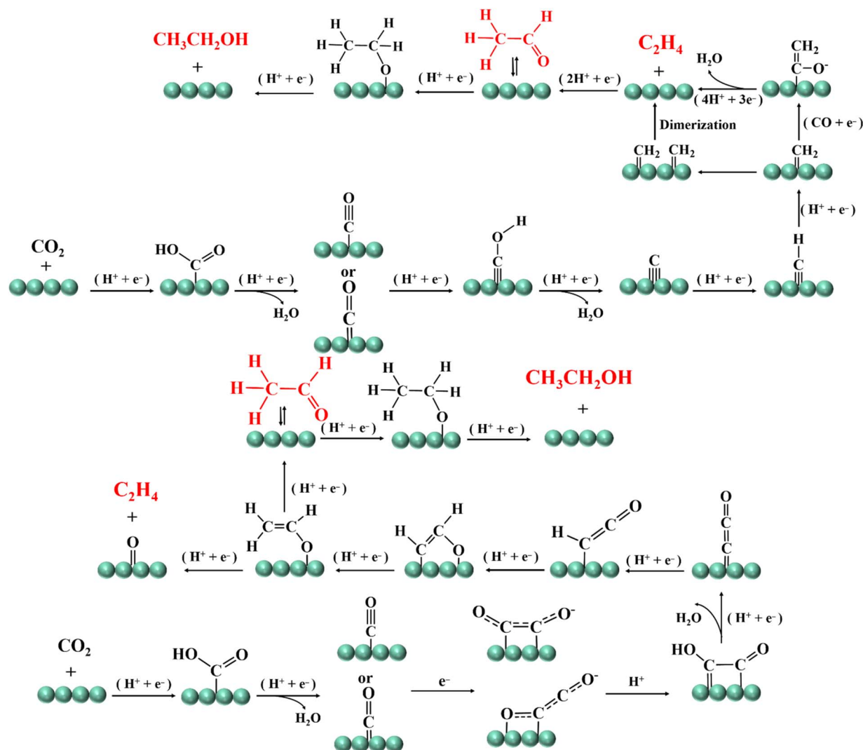
Fig. 4 Mechanism diagram of C_2 formation.
