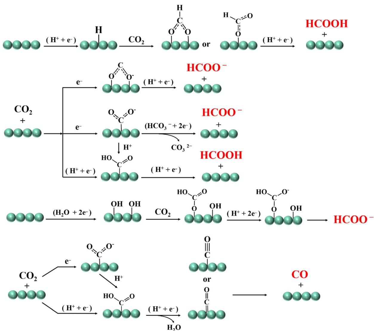
Fig. 2 Mechanism diagram of HCOO - /HCOOH and CO formation.
