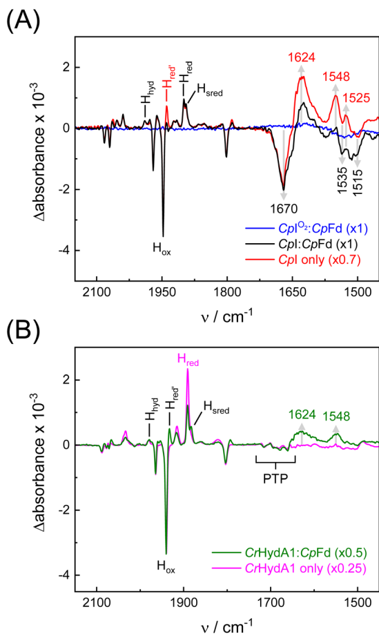
Fig. 5 Infrared difference spectroscopy. (A) \text{H}_2\text{-N}_2 ATR FTIR difference spectra of Y3pCNF- CpFd:CpI (black) and CpI alone (red) after 25 s. Bands above 1750\text{ cm}^{-1} are assigned to H-cluster ligands in the H_{\text{ox}} state (negative) and various reduced states (positive). At lower frequencies, the 1670/1624\text{ cm}^{-1} down-shift in the amide I regime indicates protein structural changes, alongside up-shifts at 1535/1548\text{ cm}^{-1} and 1515/1525\text{ cm}^{-1} . The blue spectrum serves as a negative reference where CpI was inactivated with \text{O}_2 ahead of the reaction with \text{H}_2 . (B) \text{H}_2\text{-N}_2 ATR FTIR difference spectra of Y3pCNF- CpFd:CrHydA1 (green) and CrHydA1 alone (magenta) after 50 s. Note the lack of the difference features in CrHydA1 in the amide I regime while only small changes are observed in the presence of Y3pCNF- CpFd . "PTP" refers to small difference features explored earlier. 62 All spectra are normalized to the main CO band of H_{\text{ox}} ( 1947\text{ cm}^{-1} in CpI , 1940\text{ cm}^{-1} in CrHydA1 ) with factors as indicated in the legends.
