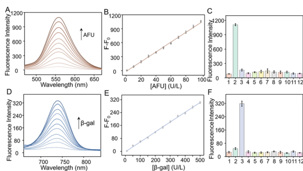
Fig. 1 The changes of fluorescence spectra of the HDQ-NA-AFU-Gal probe for \beta -gal (5–500 U per L) and AFU (1–100 U per L) in DMSO:PBS buffer (1:9, v/v). Fluorescence spectra of HDQ-NA-AFU-Gal against (A) AFU and (D) \beta -gal, respectively. Corresponding linear response of the probe against (B) AFU and (E) \beta -gal, respectively. Selectivity of the probe for (C) AFU and (F) \beta -gal at emission wavelengths of 550 nm and 740 nm, respectively. (1) Blank, (2) AFU (100 U per L), (3) \beta -gal (500 U per L), (4) esterase (0.5 U \text{mL}^{-1} ), (5) BSA (100 \mu\text{g mL}^{-1} ), (6) ALP (1 U \text{mL}^{-1} ), (7) Cys (1 mM), (8) GSH (1 mM), (9) Hcy (1 mM), (10) HClO (100 \mu\text{M} ), (11) \text{NO}_2^- (100 \mu\text{M} ), and (12) \text{H}_2\text{O}_2 (100 \mu\text{M} ).
