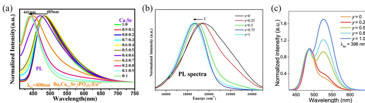
Fig. 4 (a) Normalized PL spectra of \text{Ba}_2\text{Ca}_{1-x}\text{Sr}_x(\text{PO}_4)_2:\text{Eu}^{2+} . Reproduced with permission from ref. 113. Copyright 2020, Elsevier. (b) PL spectra of the phosphors \text{Ca}_{1.98}(\text{Al}_{1-x}\text{Mg}_x)(\text{Al}_{1-x}\text{Si}_{1+x})\text{O}_7:0.02\text{Eu}^{2+} ( x = 0, 0.25, 0.5, 0.75, \text{ and } 1 ) as a function of x . Reproduced with permission from ref. 116. Copyright 2015, ACS. (c) Normalized PL spectra of \text{CsKNa}_{1.98-y}\text{Li}_y(\text{Li}_3\text{SiO}_4)_4:0.02\text{Eu}^{2+} ( 0 \leq y \leq 1 ). Reproduced with permission from ref. 76. Copyright 2019, ACS.
