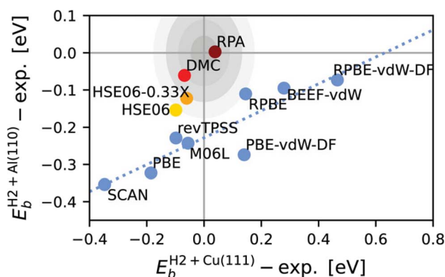
Fig. 8 Lowest reaction barrier heights for \text{H}_2 + \text{Al}(110) vs. those for \text{H}_2 + \text{Cu}(111) , both taken relative to the best semi-empirical values, as obtained with DFs including semi-local exchange (i.e., not including exact exchange, indicated by blue symbols), with screened hybrid DFs (yellow and orange symbols), with diffusion Monte-Carlo (red symbol) and with the RPA (maroon symbol). The concentric gray shaded ellipses indicate areas that would be circles in an equal-distanced representation, with radii of 1 (darkest grey), 2, 3, and 4 (lightest grey) \text{kcal mol}^{-1} respectively. For details see ref. 58. Figure reprinted from B. Oudot, K. Doblhoff-Dier, Journal of Chemical Physics , vol. 161, Article ID 054708, 2024; licensed under a Creative Commons Attribution (CC-BY) license.
