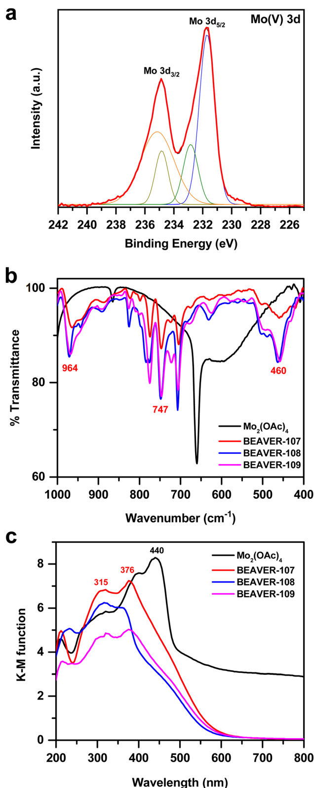
Fig. 2 Spectroscopic features of the Mo(v)-MOP molecule. (a) X-ray photoelectron spectra of BVR-107. (b) Fourier-transform infrared and (c) ultraviolet-visible spectra of \text{Mo}_2(\text{OAc})_4 , BVR-107, BVR-108, and BVR-109. All sets of spectra were recorded on the respective solids.
