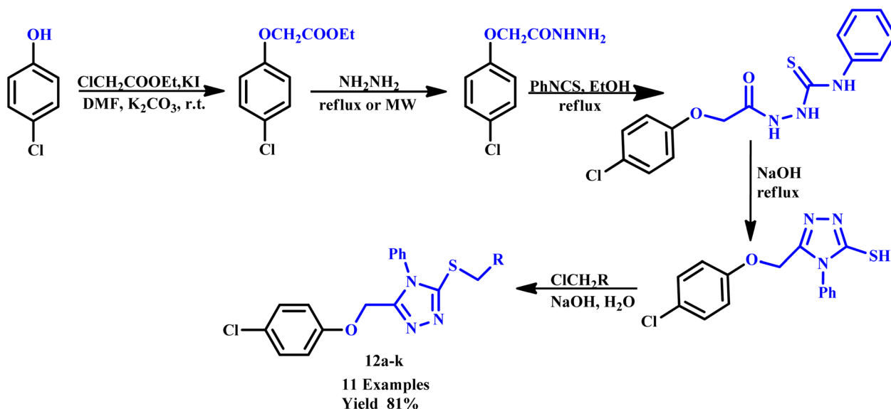
Scheme 7 Synthetic route of thioether derivatives containing 1,2,4-triazole moieties ( 12a-k ). 40
