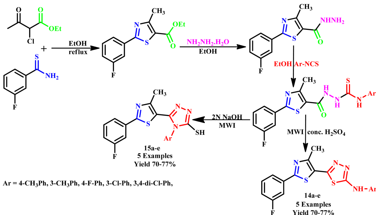
Scheme 9 . Synthetic route of {5-[2-(3-fluorophenyl)-4-methylthiazol-5-yl]-4-phenyl-4 H -1,2,4-triazole-3-thiol or 5-[2-(3-fluorophenyl)-4-methylthiazol-5-yl]- N -phenyl-1,3,4-thiadiazole-2-amine} [14a–e and 15a–e]. 44
