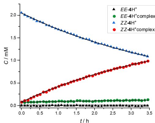
Fig. 6 Time-dependent concentration profiles of ZZ\text{-}4\text{H}^+\text{C}2 (red dots), ZZ\text{-}4\text{H}^+ (blue triangles), EE\text{-}4\text{H}^+\text{C}2 (green dots) and EE\text{-}4\text{H}^+ (black triangles). The black lines represent the fitting of the traces. The total concentrations of the axle and the macrocycle, determined from the ^1\text{H} NMR spectra ( \text{CD}_3\text{CN} , 500 MHz, 298 K) are 2.2 mM and 24 mM, respectively.
