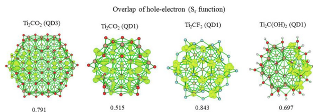
Fig. 7 Spatial map of the hole–electron overlap S_r(r) for the first optical transition, together with the corresponding S_r index, presented for the selected QDs. The isosurface value is 0.001 \text{ e} \text{ \AA}^{-3} .
