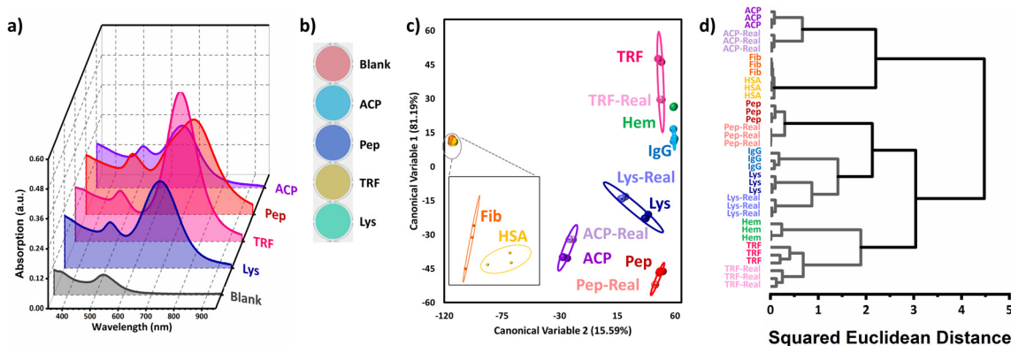
Fig. 7 (a) Spectral variation, (b) corresponding image responses, (c) 2D LDA score plot and (d) HCA dendrograms obtained using the Ward method of the colorimetric multidimensional probe in the presence of proteins in real urine samples.
