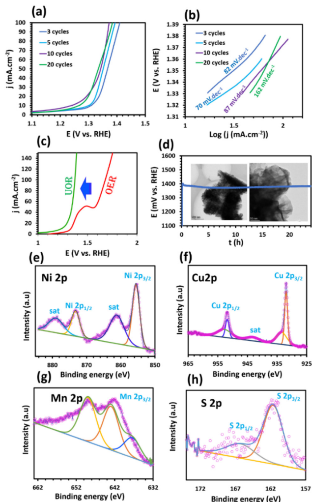
Fig. 4 (a) and (b) LSV and corresponding Tafel curves of the electrodes fabricated at different cycles for UOR in 1.0 M KOH + 0.33 M urea solution, (c) comparison of OER and UOR of the Ni-Mn-S/Ni-Cu/10 sample, (d) CP curve for the evaluation of the electrocatalytic stability of the optimized sample at 100 \text{ mA cm}^{-2} (TEM images after the stability test). High-resolution XPS spectra of the Ni-Mn-S/Ni-Cu/10 sample after the UOR stability test: (e) Ni 2p, (f) Cu 2p, (g) Mn 2p, and (h) S 2p.
