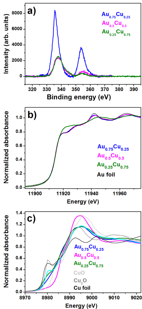
Fig. 3 (a) XPS core level Au 4d spectra recorded for Au_xCu_{1-x} /TNTs ( x = 0.75, 0.5, and 0.25 ). XANES spectra of (b) Au- L_3 edge and (c) Cu K-edge.
