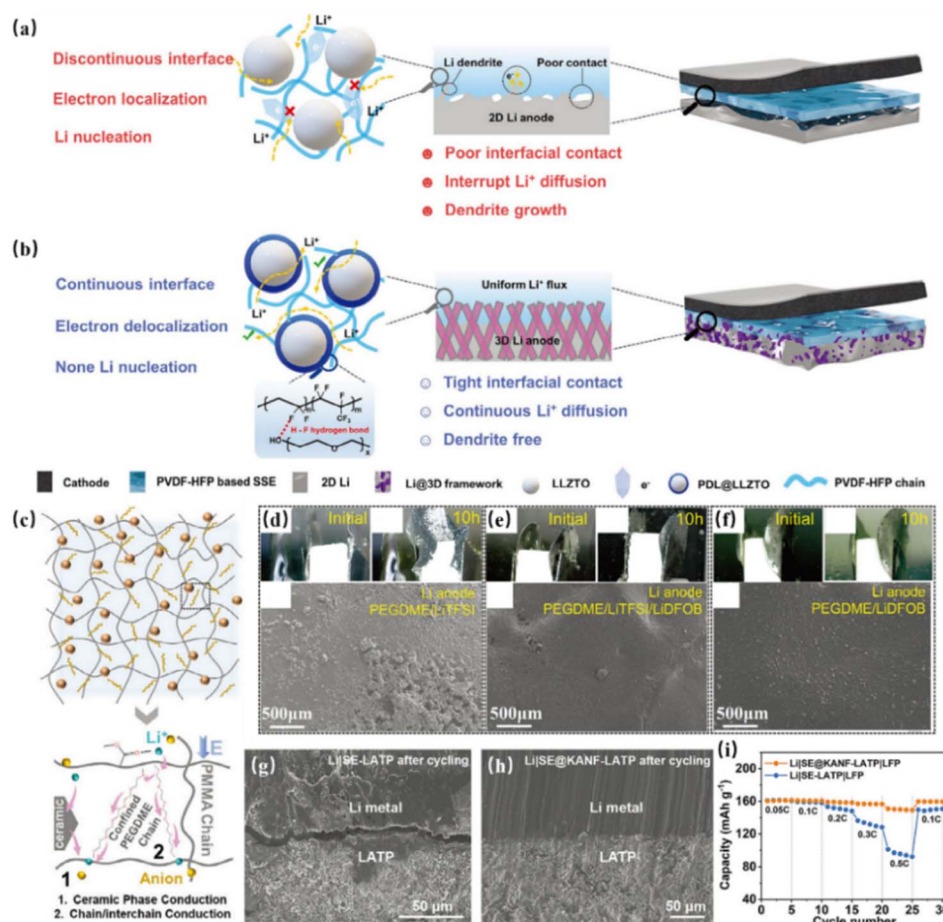
Fig. 4 (a) Schematic of Li ^{+} transport and charge distribution at the electrolyte–electrode interface in LLZTO and (b) PDL@LLZTO effect of electrolyte on 2D/3D lithium anodes. 57 (c) Diagram of the PEGDME@PMMA electrolyte and internal Li ^{+} transport. 54 Digital photos and SEM of lithium deposition before cycling and after 10 hours for (d) PEGDME/LiTFSI, (e) PEGDME/LiTFSI/LiDFOB, and (f) PEGDME/LiDFOB. 54 SEM of cross-sections after cycling of (g) Li|SE-LATP and (h) Li|SE@KANF-LATP. 53 (i) Performance of Li|SE@KANF-LATP|LFP and Li|SE-LATP|LFP. 53
