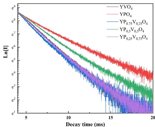
Fig. 8 Luminescence decay curves for Y(P_{1-x}V_x)O_4:5\% \text{ Eu} .
