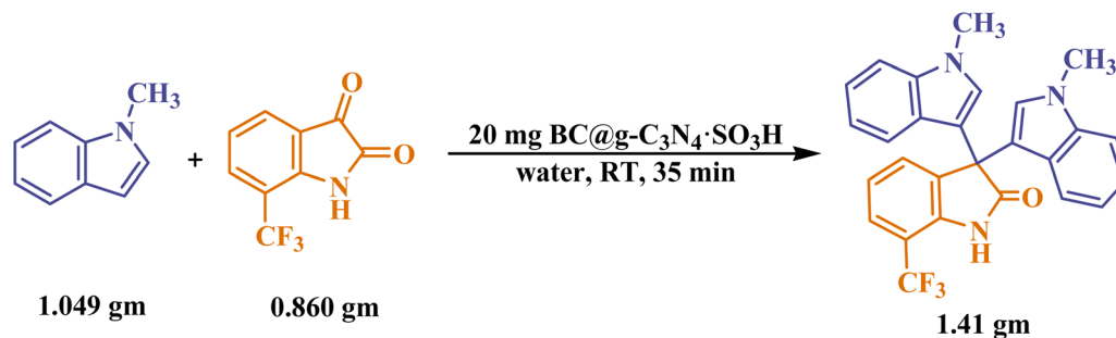
Scheme 3 The scale-up synthesis of 7- \text{CF}_3 -isatin and indole-derived bis-indole.
