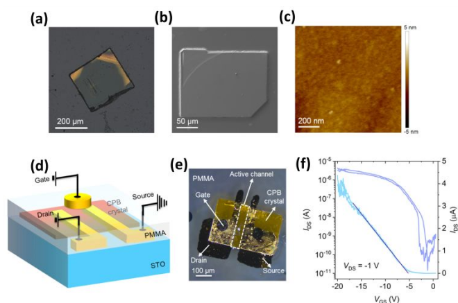
Fig. 5 (a) Optical image depicting the CPB single crystal, characterized by a regular rectangular shape, positioned on the \text{SrTiO}_3 substrate. (b) Top-view SEM image of the \text{CsPbBr}_3 single crystal. (c) Tapping-mode AFM topography imaging reveals the smooth and uniform surface of the epitaxially grown single crystal. (d) Diagram illustrating the structure of the FET. (e) Top view of the FET device utilizing a \text{CsPbBr}_3 single crystal, incorporating PMMA as the gate dielectric. (f) Dual-sweep transfer curves of the FET at a source-drain voltage of -1 V. Reprinted with permission. 105 Copyright 2021, American Chemical Society.
