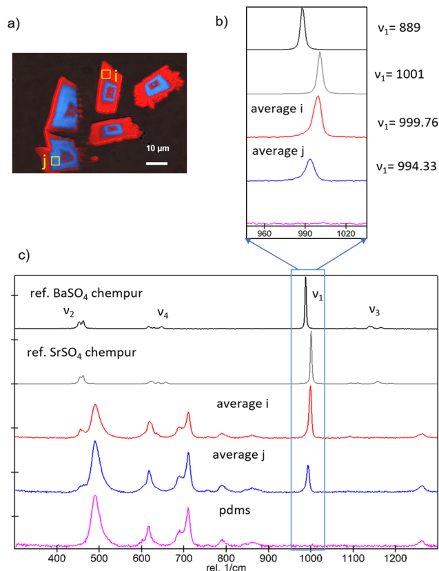
Fig. 11 a) Raman oscillatory zoned crystal of (\text{Ba}_x\text{Sr}_{1-x})\text{SO}_4 with Sr (in red) enriched and Ba (in blue) enriched solid solution. b) and c) Raman signature of reference \text{BaSO}_4 (barite) and \text{SrSO}_4 (celestine) and the newly formed phases (i) and (j) with (b) zoom on the prominent sulfate band and (c) the complete spectra. Reproduced from Poonoosamy et al. 116 with permission from Springer Nature, copyright 2021.
