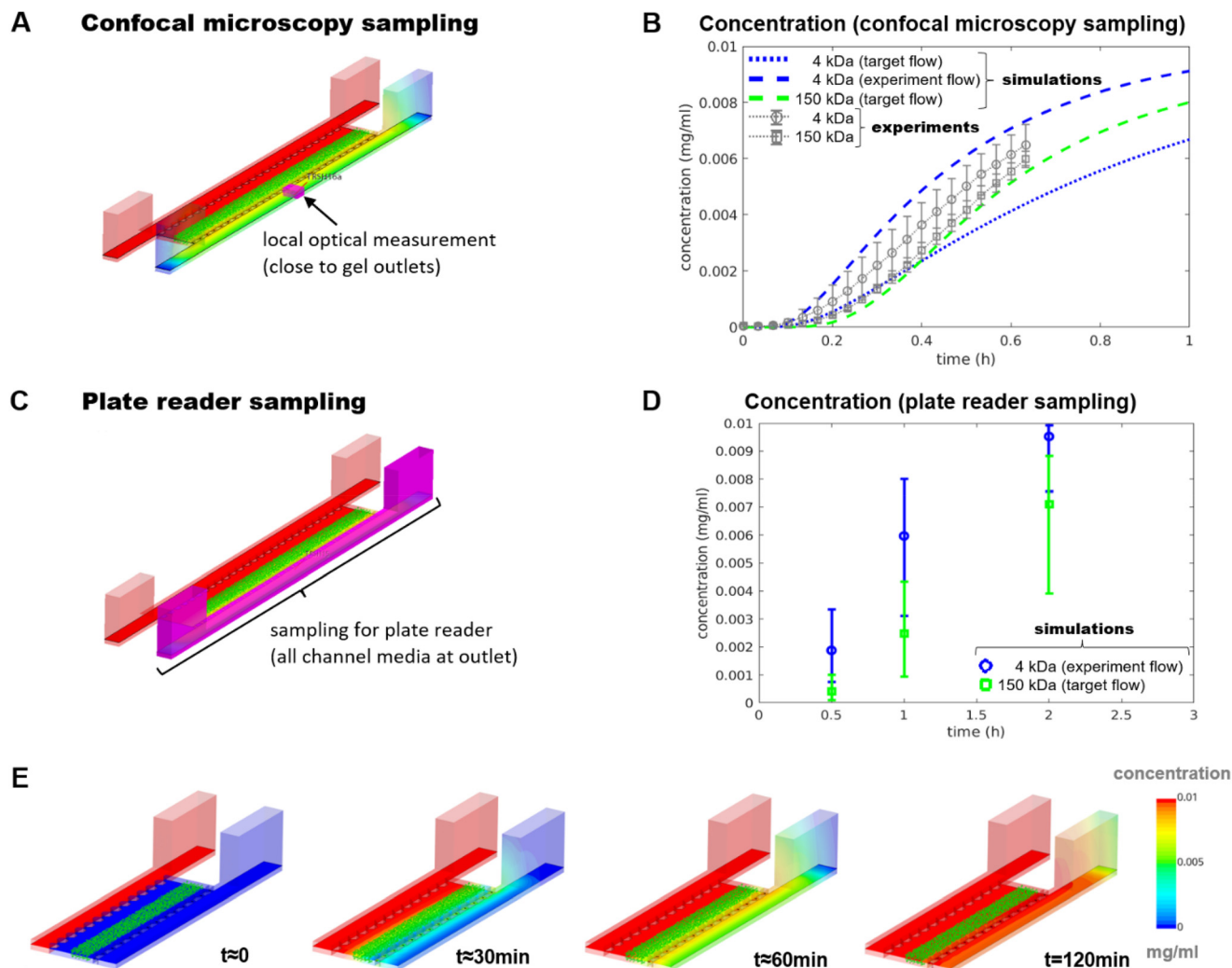
Fig. 3 Computational fluid dynamics (CFD) simulations for prediction of time–concentration profiles. (A) Schematic depicting confocal microscopy sampling. (B) Concentration–time profiles derived from confocal sampling (corresponding experimental data can be found in Table S6–S9†). (C) Schematic depicting plate reader sampling. (D) Concentration–time profiles derived from plate reader sampling. (E) Spatial molecule mass concentration at four different time points ( t \approx 0, 0.5, 1.0 and 2.0 h).
