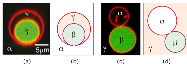
Fig. 15 Complete engulfment of condensate droplets by a membrane (red): (a and b) two-sphere shape of the membrane, which completely engulfs the dextran-rich \beta droplet (green) via an in-bud and forms a closed membrane neck adjacent to the droplet; reused with permission from ref. 71, American Chemical Society, 2012 (c and d) two-sphere shape of the membrane, which forms two spherical segments around both the dextran-rich \beta (green) and the PEG-rich \alpha (black) droplet, connected by a closed membrane neck 72 In both cases, the system's free energy is strongly reduced by eliminating the \alpha\beta interface.
