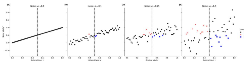
Fig. 4 Uniformly distributed synthetic datasets of size N = 50 , with no added noise (a), Gaussian noise added with standard deviations of \sigma_E = 0.1 (b), \sigma_E = 0.25 (c), and \sigma_E = 0.5 (d). If we consider the classification case, the boundary b is shown as a vertical dashed line. Resulting false negatives (fn) and false positives (fp) due to addition of noise are colour coded. Predictor noise \sigma_{\text{pred}} = 0 for all cases.
