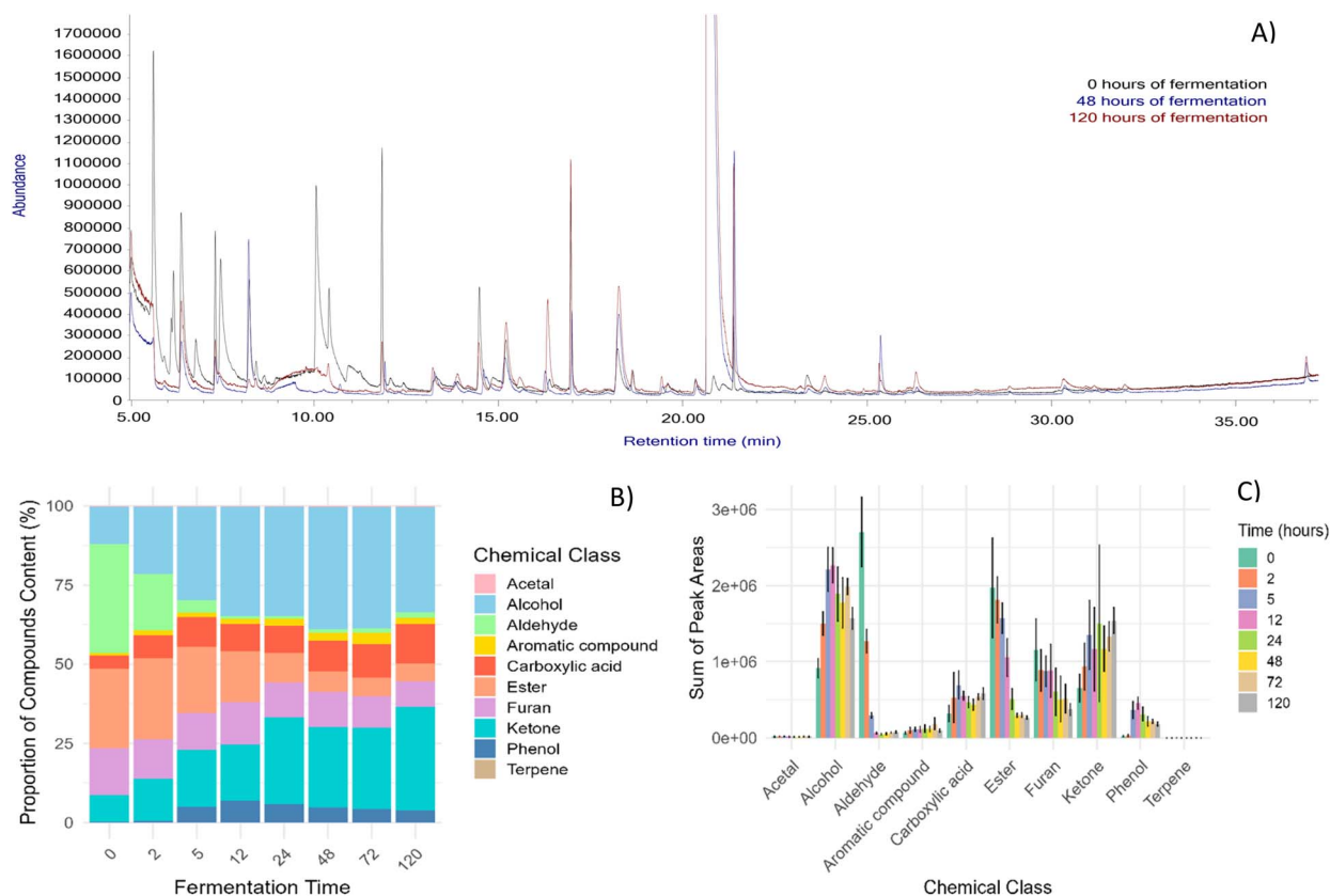
Fig. 2 Changes in oat volatiles over the course of 120 h of solid-state fermentation. (A) Overlaid chromatogram of 0 (black), 48 (blue), and 120 (red) h of SSF of oats. (B) Summed proportions of peak areas for each chemical class at each sampled timepoint. (C) Dynamic changes in chemical class peak areas at each sampled timepoint. Error bars denote standard deviations.
