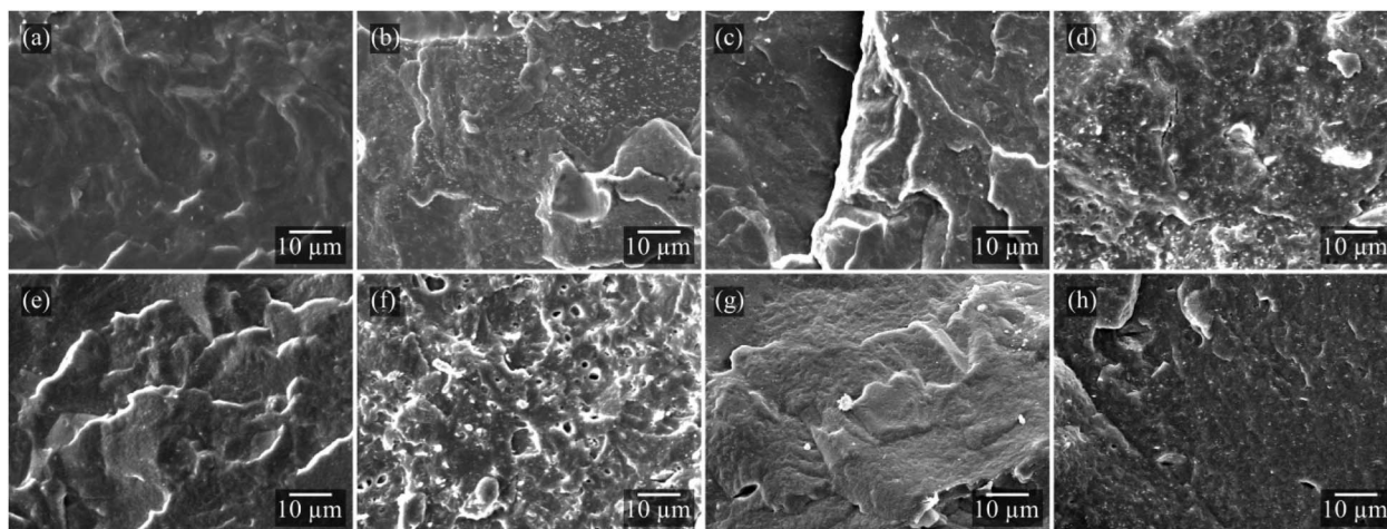
Fig. 3 SEM micrographs of (a) P, (b) PSep, (c) PO, (d) POSeq, (e) PR, (f) PRSep, (g) PB, and (h) PBSeq compositions.
