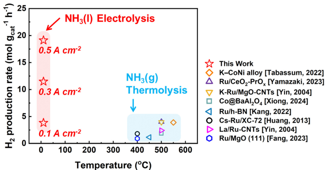
Fig. 4 Comparison of H_2 production rate ( mol\ g_{cat}^{-1}\ h^{-1} ) obtained by NH_3(l) electrolysis and NH_3(g) thermolysis. The unit mass of a catalyst for NH_3(l) electrolysis is defined as the mass of the catalyst of the cathode (12.2 mg of Pt/C).
