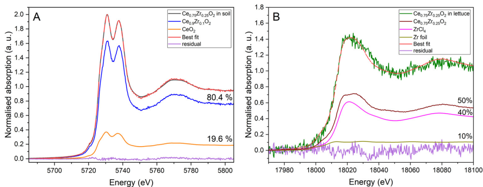
Fig. 4 (A) Ce L_3 -edge normalised XANES spectrum of Ce_{0.75}Zr_{0.25}O_2 treated soil samples and best linear combination fit of XANES profiles of Ce_{0.9}Zr_{0.1}O_2 and CeO_2 . (B) Zr K-edge normalised XANES spectrum of Ce_{0.75}Zr_{0.25}O_2 grown lettuce tissue and best linear combination fit of XANES profiles of pristine Ce_{0.75}Zr_{0.25}O_2 and ZrCl_4 and Zr metal foil.
