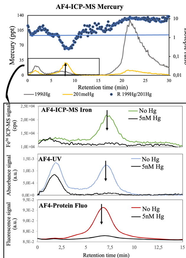
Fig. 5 Size-resolved analysis of simultaneous mercury ( ^{199}\text{iHg} ) and methyl-mercury ( ^{201}\text{MeHg} ) interactions with EPS components released by a diatom, C. meneghiniana , (A) and a cyanobacterium, Synechocystis sp., (B) using AF4-ICP-MS and UV-Fluo. The isotopic ratio is present as the log of ( ^{199}\text{iHg}/^{201}\text{MeHg} ). The ratio increased as iHg bound to EPS increased compared with MeHg ( >1 ), but decreased when MeHg bound to EPS increased compared with iHg ( <1 ). The UV-vis scans, obtained at different retention times with AF4-MD (labelled 1, 2 and 3) are presented, allowing the identification of hemic protein with Soret absorption band (*) eluting mainly at retention time 2. Fractionation conditions and settings are provided in ESI ^{\dagger} section S4 (unpublished data).
