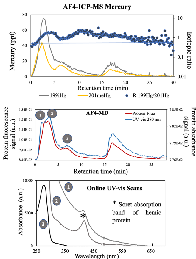
Fig. 5 Size-resolved analysis of simultaneous mercury ( ^{199}\text{iHg} ) and methyl-mercury ( ^{201}\text{MeHg} ) interactions with EPS components released by a diatom, C. meneghiniana , (A) and a cyanobacterium, Synechocystis sp., (B) using AF4-ICP-MS and UV-Fluo. The isotopic ratio is present as the log of ( ^{199}\text{iHg}/^{201}\text{MeHg} ). The ratio increased as iHg bound to EPS increased compared with MeHg ( >1 ), but decreased when MeHg bound to EPS increased compared with iHg ( <1 ). The UV-vis scans, obtained at different retention times with AF4-MD (labelled 1, 2 and 3) are presented, allowing the identification of hemic protein with Soret absorption band (*) eluting mainly at retention time 2. Fractionation conditions and settings are provided in ESI ^{\dagger} section S4 (unpublished data).
