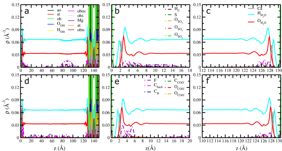
Fig. 2 Computed atomic density profiles (ADPs) of 6:2 FTS and 6:2 FTC and H 2 O molecules as a function of the distance normal to the basal surface of montmorillonite. (a–c) 6:2 FTS (d–f) 6:2 FTC. The O H 2 O and H H 2 O are shown as solid red and cyan. Dashed lines represent the atoms of 6:2 FTS/6:2 FTC molecules. The O SO 3 and S SO 3 represent oxygen and sulfur atoms in 6:2 FTS and the O COO and C COO represent oxygen and carboxyl carbon atoms in 6:2 FTS. The C back , F and H C corresponds to carbon backbone, fluorine and hydrogens in each FT’s. Labels – ao, at, st, ob, obts, obos and ohs represent surface atoms in montmorillonite following the notation used in clayff. 55 The origin ( z = 0) is the mean position of the basal surface ‘O’ atoms of montmorillonite.
