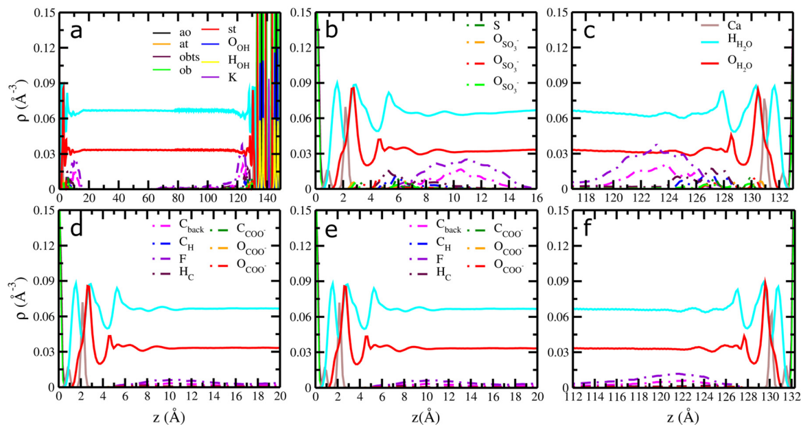
Fig. 3 Computed atomic density profiles (ADPs) of 6:2 FTS and 6:2 FTC and H 2 O molecules as a function of the distance normal to the basal surface of illite. (a–c) 6:2 FTS (d–f) 6:2 FTC. The O H 2 O and H H 2 O are shown as solid red and cyan. Dashed lines represent the atoms of 6:2 FTS/6:2 FTC molecules. The O SO 3 and S SO 3 represent oxygen and sulfur atoms in 6:2 FTS and the O COO and C COO represent oxygen and carboxyl carbon atoms in 6:2 FTS. The C back , F and H c corresponds to carbon backbone, fluorine and hydrogen in each FT's. Labels – ao, at, st, ob, and obts represent surface atoms in montmorillonite following the notation used in clayff. 55 The origin ( z = 0 ) is the mean position of the basal surface 'O' atoms of illite.
