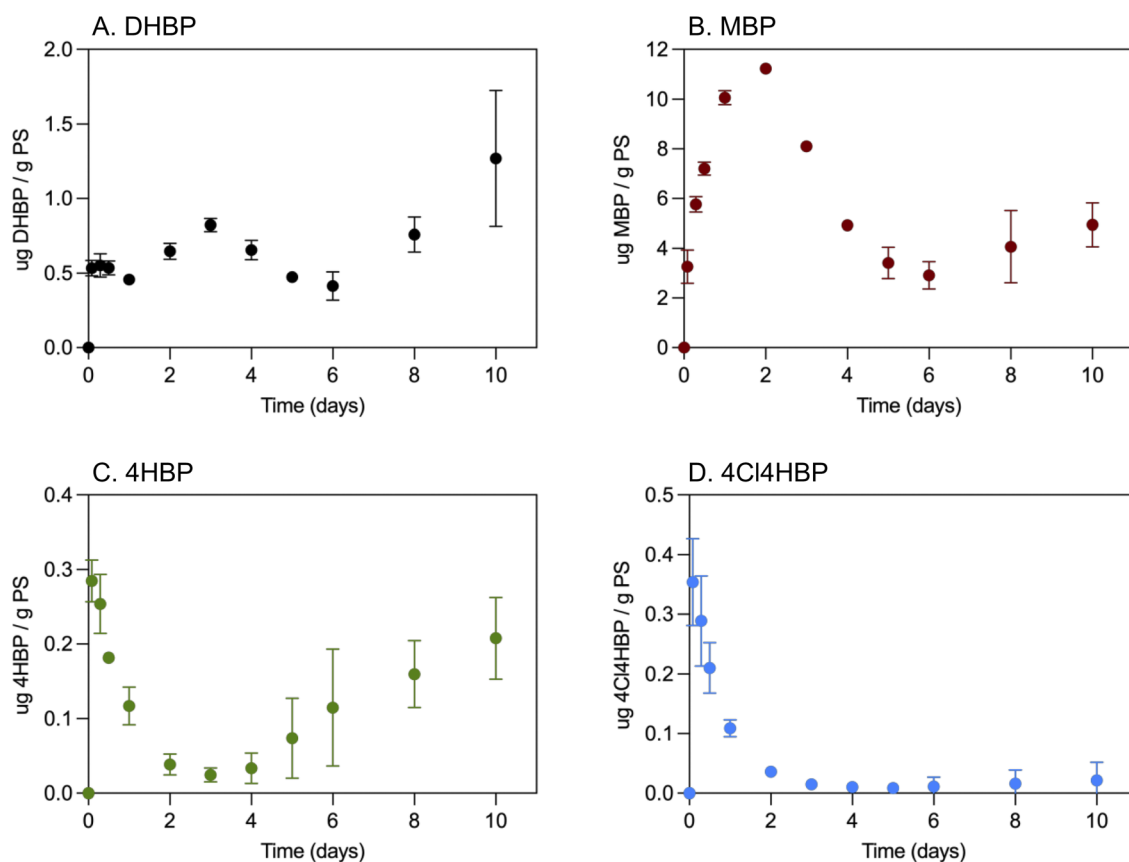
Fig. 4 Concentration of (A) DHBP, (B) MBP, (C) 4HBP, and (D) 4Cl4HBP detected in the leachate of 1 w/w% benzophenone-PS composites ( n = 2 ) suspended in water and exposed to \text{UV}_{>300\text{nm}} irradiation.
