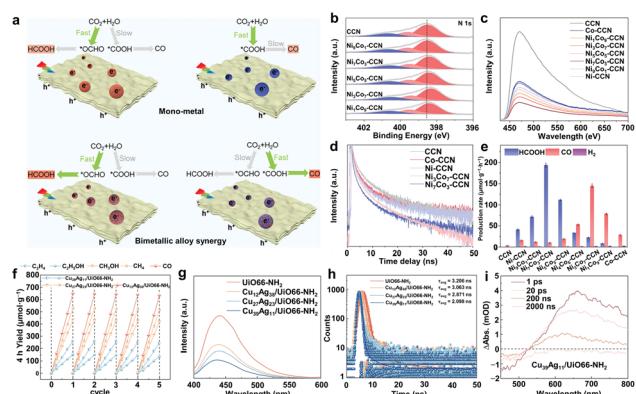
Fig. 5 (a) Schematic diagram of the reaction mechanism of photoreduction of CO 2 by the Ni x Co y -CCN catalyst. (b) XPS spectra of N 1s, (c) PL spectra and (d) time-resolved transient PL decay spectra for Ni x Co y -CCN. (e) Product evolution rates of Ni x Co y -CCN. Reproduced with permission from ref. 50. Copyright 2024, Wiley-VCH. (f) The cycling test over Cu x Ag 50-x /UiO66-NH 2 . (g) PL spectra; (h) time-resolved transient PL decay spectra and (i) Fs-TA spectra of Cu x Ag 50-x /UiO66-NH 2 . Reproduced with permission from ref. 51. Copyright 2024, Royal Society of Chemistry.
