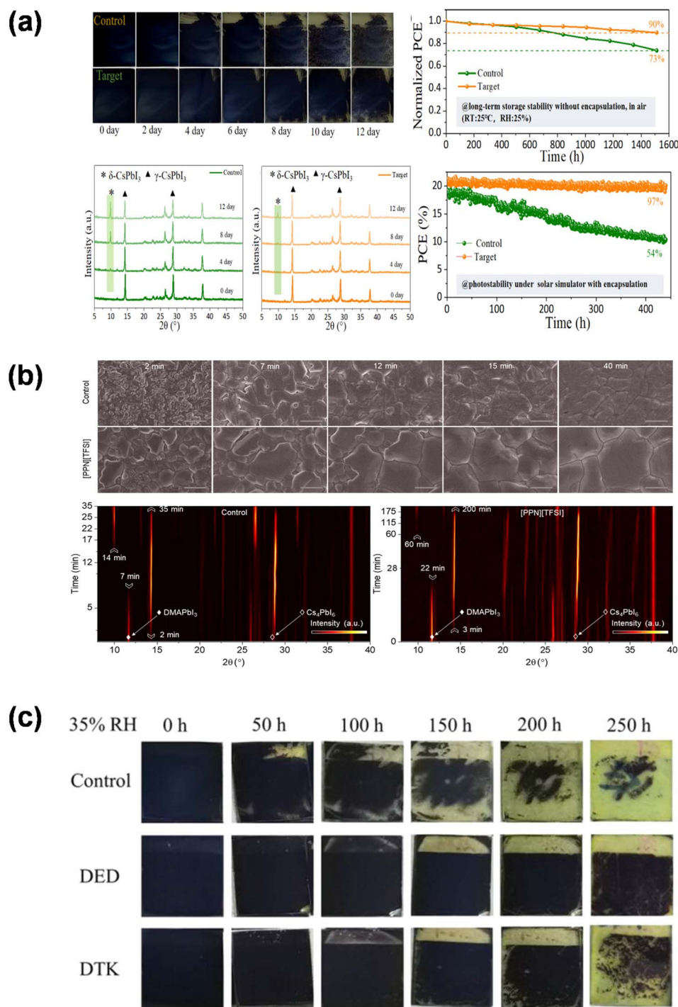
Fig. 10 The review of stability enhancement via additive engineering with (a) CSE in CsPbI 3 perovskite (reproduced with permission from ACS Energy Lett., 9(10), 4817–4826. Copyright 2024 American Chemical Society), 103 (b) [PPN][TFSI] in CsPbI 3 , 86 and (c) DED in CsPbI 3 (reproduced with permission from Adv. Mater., 35(12), 2210223. Copyright 2023 Wiley-VCH GmbH). 93
