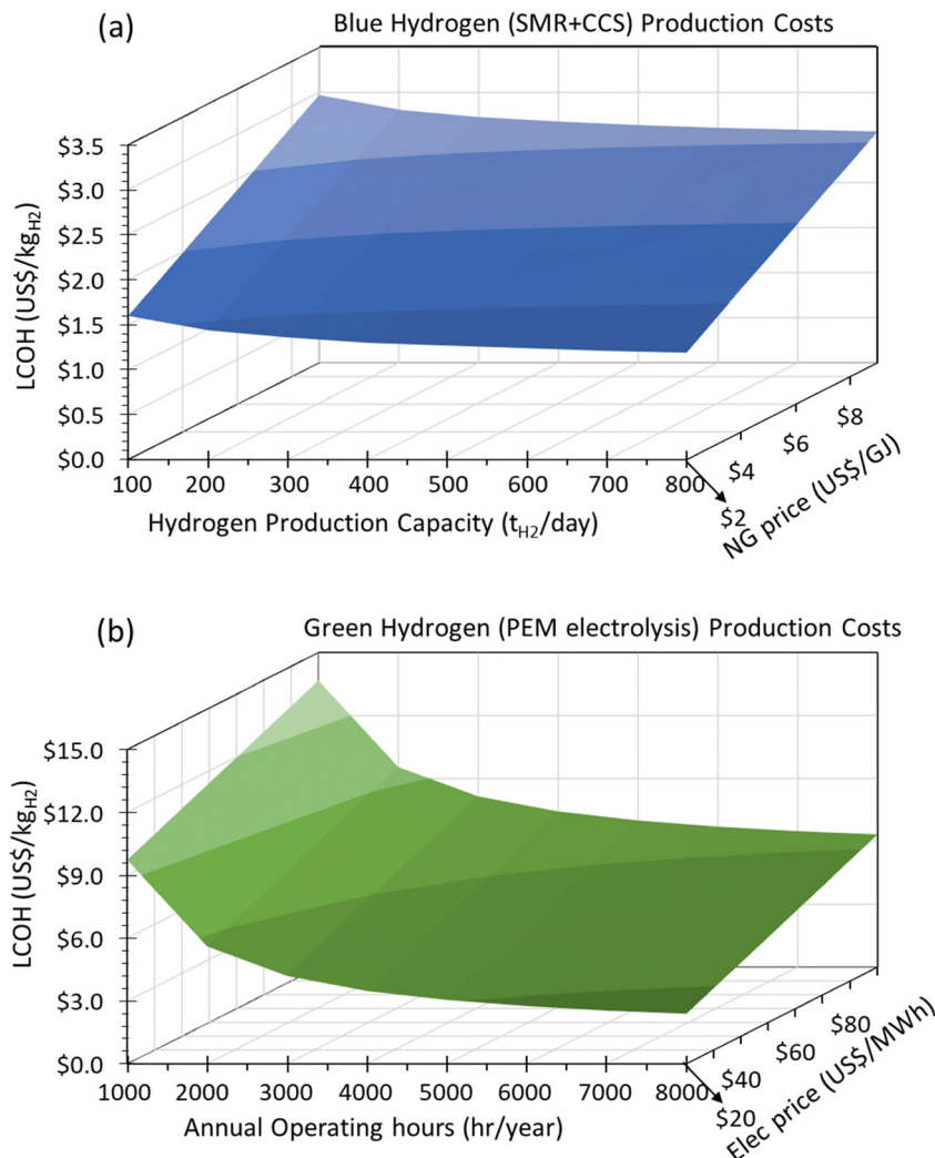
Fig. 5 (a) Levelized cost of blue hydrogen ($ per kg H 2 ) produced via SMR + CCS as a function of natural gas price ($ per GJ) and plant size (t H 2 per day). (b) Levelized cost of green hydrogen ($ per kg H 2 ) produced via PEM electrolysis as a function of electricity price ($ per MWh) and annual operating hours (hours per year).
