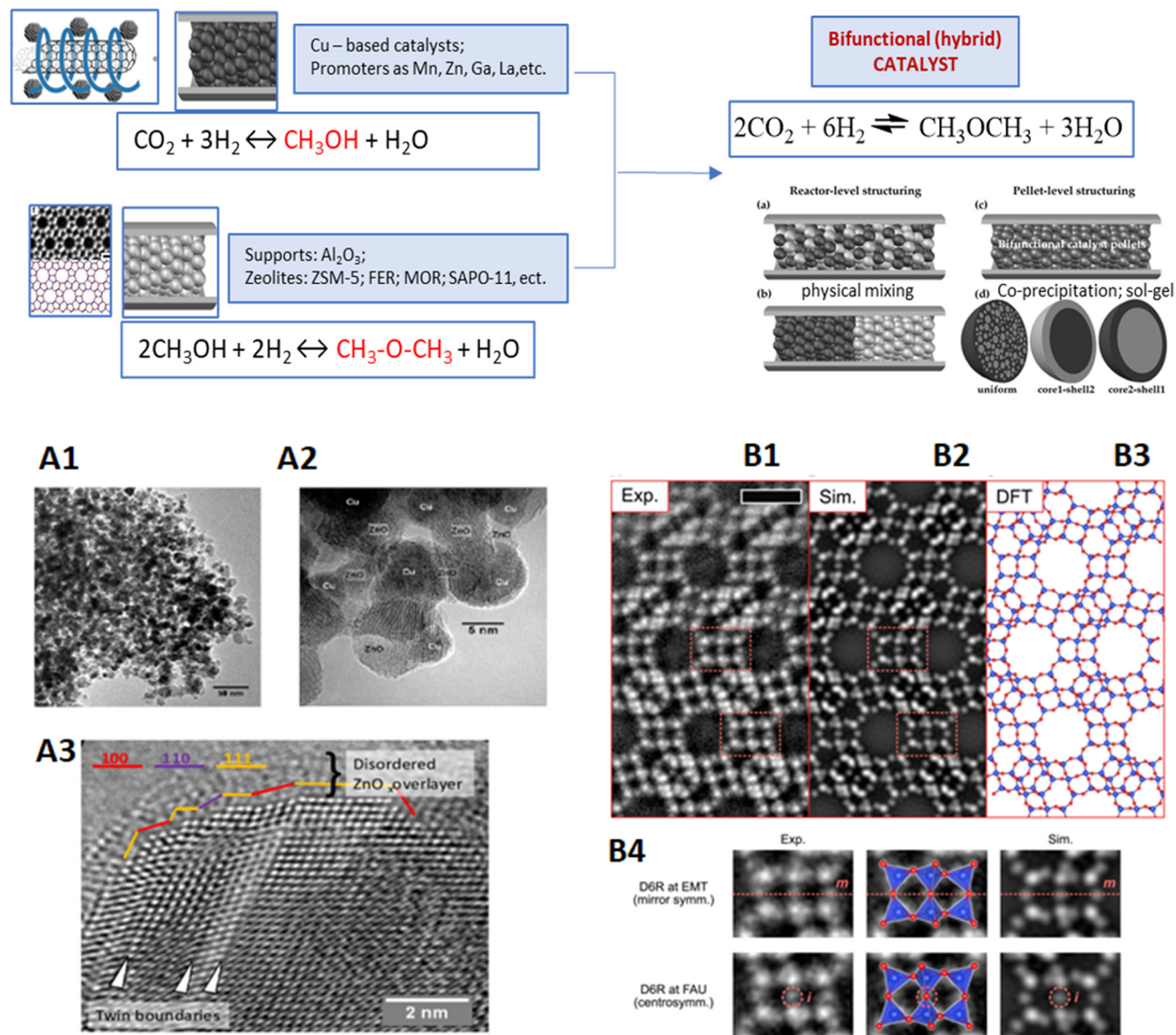
Fig. 6 Studied designed catalysts for DME synthesis. Conventional catalysts for DME synthesis from syngas. A – HRTEM images of a Cu/ZnO/Al 2 O 3 ; A1 – porous aggregates of metallic Cu and ZnO, A2 – Cu/ZnO/Al 2 O 3 nanoparticles, A3 – details of the surface faceting, decoration, and defect structure, B – OBF STEM images of a zeolite catalysts: B1 – unit-cell-averaged experimental OBF image. Scale bar, 1 nm. B2 – Simulated OBF image based on the DFT-relaxed structure shown in B3. B3 – Atomic structure model of FAU twin boundary relaxed by the DFT calculation. The blue and red balls indicate the T and oxygen sites, respectively. B4 – Comparison of D6R structures on the twin boundary and bulk region. Experimental and simulated images are shown for each structure, and atomic structure models represented as a TO 4 tetrahedral configuration are overlaid. Copyright 137,138 2017 Earth and Environmental Science.
