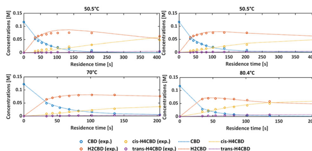
Fig. 7 Kinetic profiles for the hydrogenation of a 0.1 M solution of CBD over Pt/alumina 2 CSMs (set B), at different temperatures. Lines = fitted model; points = measured data.
