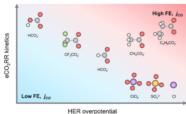
Fig. 11 Effect of electrolyte anions on ECR of \text{CO}_2 and hydrogen evolution reaction. 142
