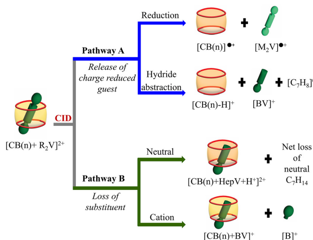
Scheme 2 Fragmentation pathways of CB–viologen complexes. Neutral CB host is shown in yellow, while the charged guest is shown in orange. The radical methyl viologen, [\text{M}_2\text{V}]^{\bullet+} , is shown in lighter green to highlight the presence of this species in comparison with other guests that are even electron ions.
