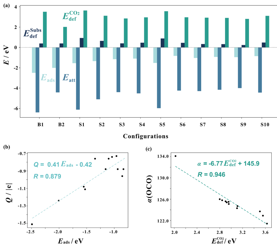
Fig. 3 (a) CO 2 adsorption on bare Mo 6 C 5 on the different sites and modes and the energy contribution breakdown; (b) Bader charge ( Q ) of adsorbed CO 2 vs. E_\text{ads} , showing the linear correlation and the regression coefficient, R ; and (c) \alpha(\text{OCO}) vs. the deformation energy of CO 2 , with the linear equation and R value.
