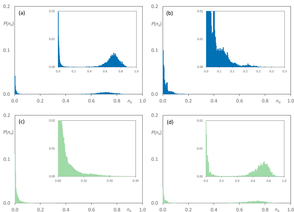
Fig. 12 Discrete probability distribution function, P(n_a) , for [C_8\text{MIM}]_{1-x}[C_8\text{MIM-F}_{13}]_x[\text{Tf}_2\text{N}] : [C_8\text{MIM}]^+ chains at (a) x = 0.35 ; (c) x = 0.5 ; [C_8\text{MIM-F}_{13}]^+ chains at (b) x = 0.35 ; (d) x = 0.5 . Reproduced from ref. 34.
