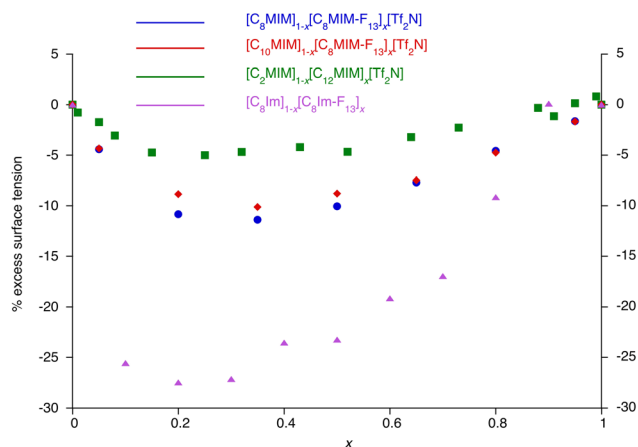
Fig. 11 Excess surface tension (%) for the mixtures [C_8\text{Im}]_{1-x}[C_8\text{Im-F}_{13}]_x , [C_8\text{MIM}]_{1-x}[C_8\text{MIM-F}_{13}]_x[\text{Tf}_2\text{N}] , [C_{10}\text{MIM}]_{1-x}[C_8\text{MIM-F}_{13}]_x[\text{Tf}_2\text{N}] and [C_2\text{MIM}]_{1-x}[C_{12}\text{MIM}]_x[\text{Tf}_2\text{N}] . 28,30,34
