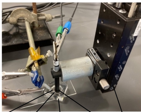
counter electrode reference electrode PDMS reservoir working electrode micrometer
